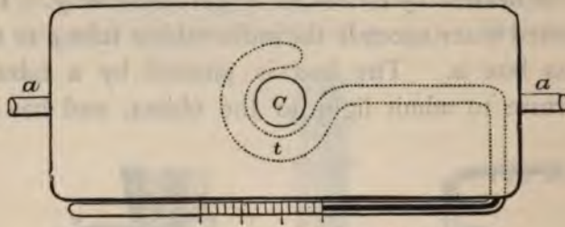
FIG. 34.—STRICKER'S WARM STAGE.
